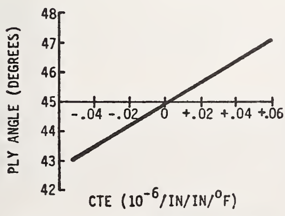
FIGURE 4 : GY-70 ISOTROPIC LAMINATE CTE SENSITIVITY
